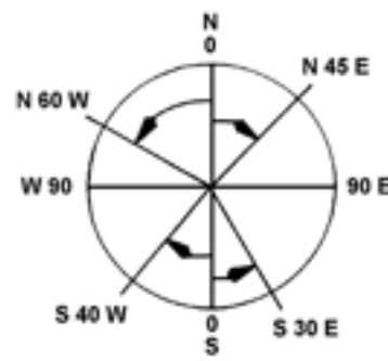
Figure 6. Bearings are read from a quadrant compass
